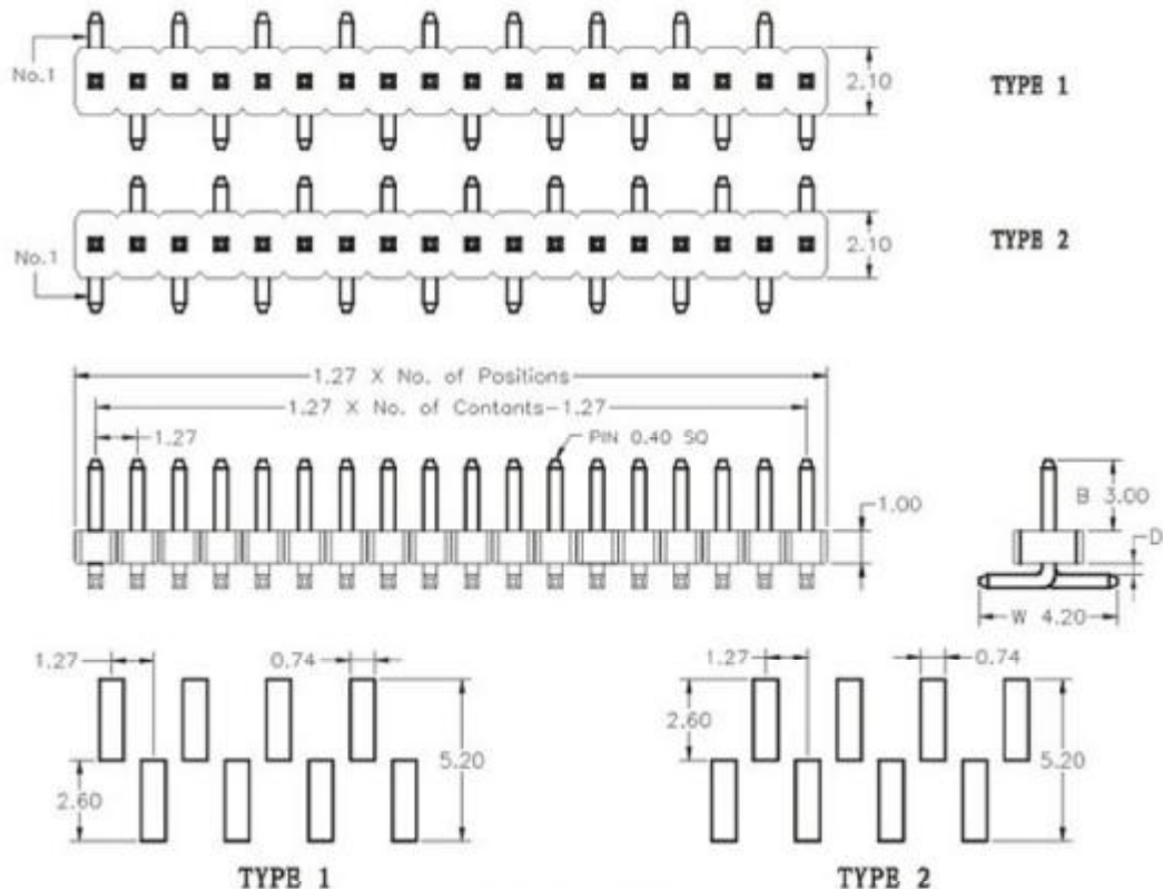
PCB LAYOUT
