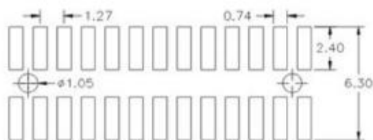
PCB LAYOUT
