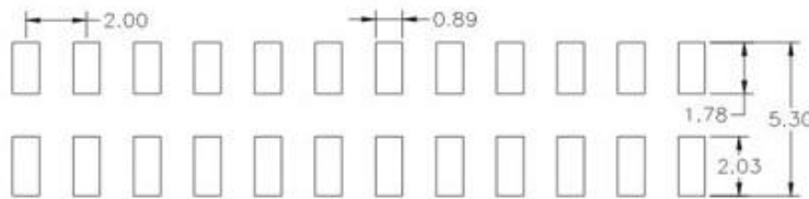
PCB LAYOUT
