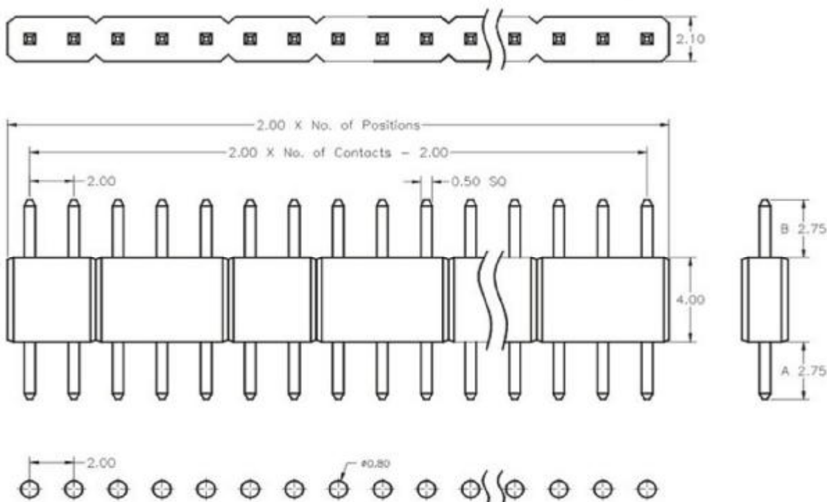
PCB LAYOUT
